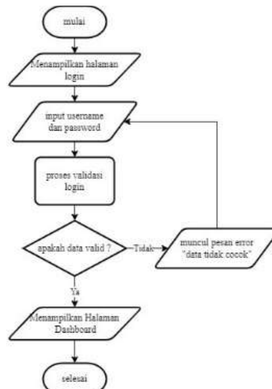
Gambar 2. Flowchart Login
