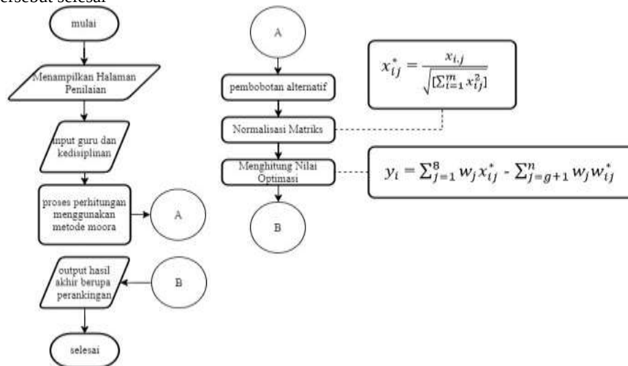
Gambar 3. Flowchart Perhitungan Metode Moora
