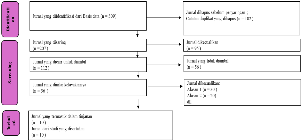
Gambar 1. PRISMA flowchart
